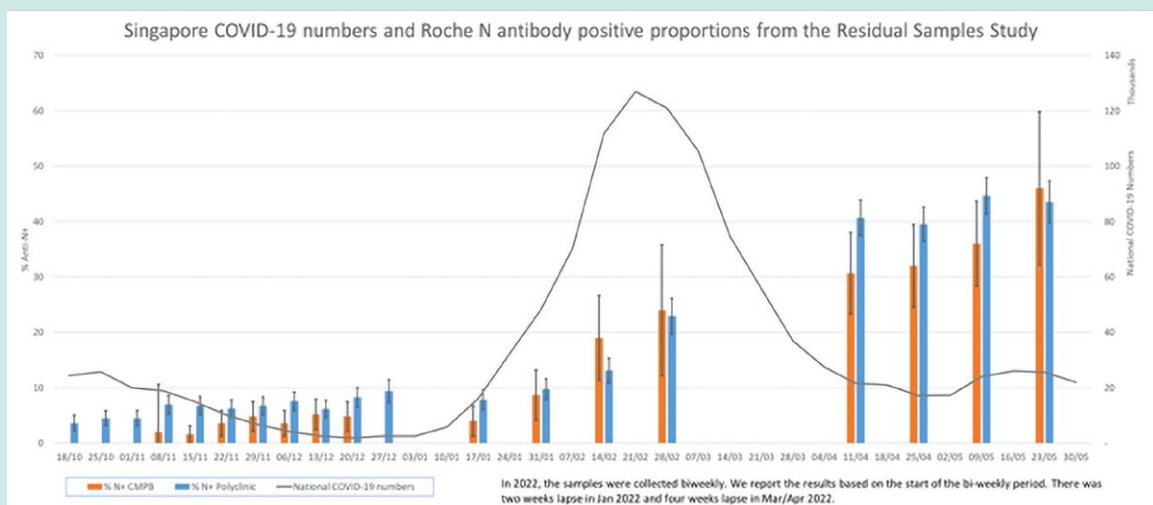
Singapore COVID-19 numbers and Roche N antibody positive proportions
